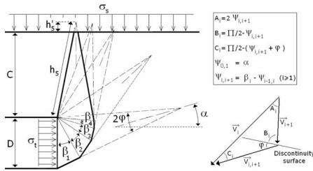
a. M1 mechanism (collapse case) in the (y, z) plane
