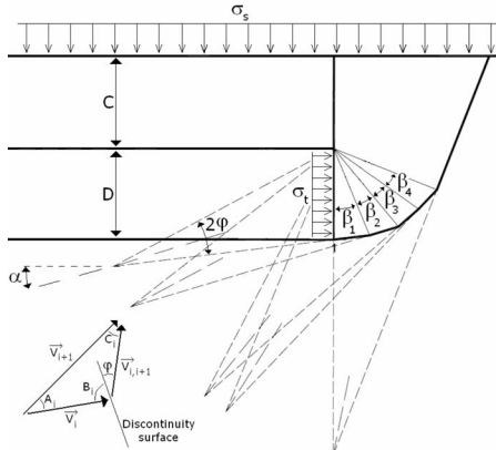
b. M2 mechanism (blow-out case) in the (y, z) plane
