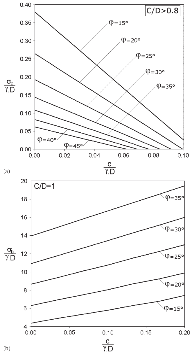
Figure 12. Design charts of the critical pressure for a frictional and cohesive soil: (a) collapse and (b) blow-out.
